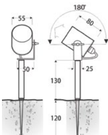
Eco adjustable with ground spike
