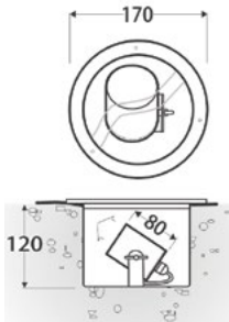
Lawn Light inground
