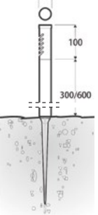
Path Light with ground spike
