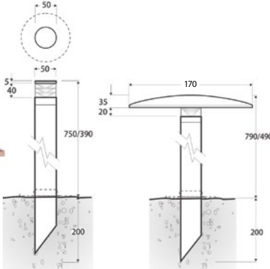
Bollard round 390 / 750mm
