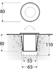
Up Light spun inground
