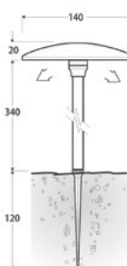
Spread Light with ground spike
