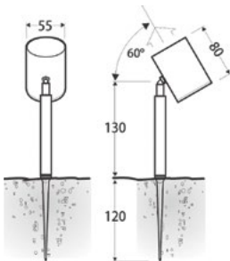
Spotlight adjustable with ground spike
