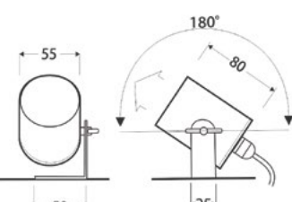
Underwater Light surface mount
