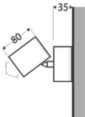
Spot Light surface endmounted adjustable
