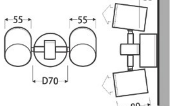
Double Spot Light surface mounted adjustable
