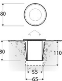
Up Light machined inground
