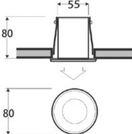
Down Light recessed
